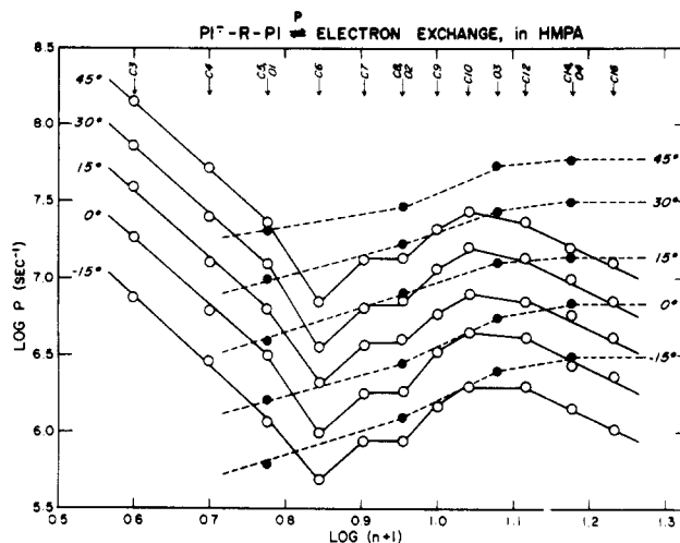
Figure 12. Dependence of the frequency P ( \text{s}^{-1} ) for intramolecular electron exchange upon the number of atoms separating the two substituents on the chain ends, in HMPA at the temperature indicated. (O) \text{PI}-(\text{CH}_2)_n\text{-PI}\cdot^- ; (●) \text{PI}-(\text{CH}_2\text{CH}_2\text{O})_m\text{CH}_2\text{CH}_2\text{PI}\cdot^- ; PI is the N -phthalimide group. From ref 107b.
