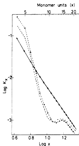
Figure 3. Molar cyclization equilibrium constants of dimethylsiloxanes at 110 °C. Values calculated from the rotational isomeric state model assuming a Gaussian end-to-end distribution (×) are compared with values measured by Semlyen 9 for equilibration in bulk (○) and values measured by Brown and Slusarczyk 28b for equilibration in toluene solution (●). Reproduced with permission from J. A. Semlyen and P. V. Wright, Polymer , 10, 543 (1969). Copyright 1969, IPC Business Press Ltd.
