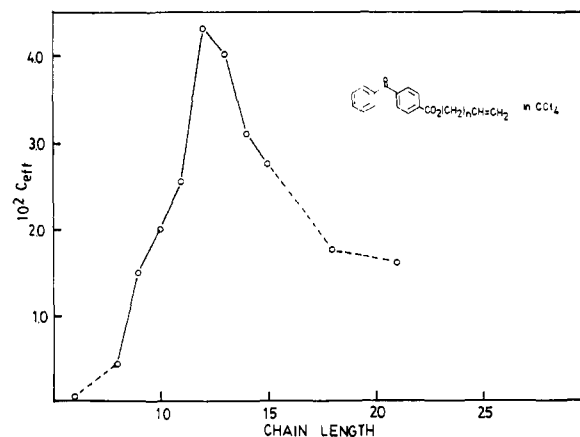
Figure 10. The rate constant for intramolecular phosphorescence quenching, k_{o,m} , by the terminal alkene group in the molecules benzophenone-4 \text{CO}_2\text{-(CH}_2\text{)}_m\text{-CH=CH}_2 , expressed as C_{eff} = k_{o,m}/k_q^{(2)} , as a function of chain length. The data were obtained from measurements in \text{CCl}_4 solution at 5 \times 10^{-4} M at 22 °C. See ref 105c.
