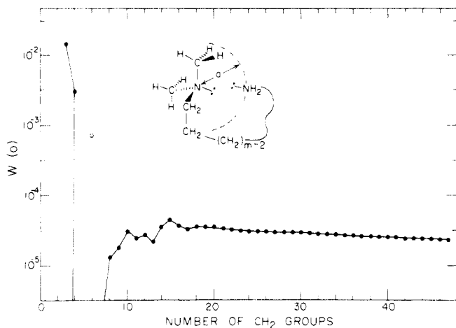
Figure 16. Calculated end-to-end cyclization probability W(O) for the molecules \text{Me}_2\text{N}(\text{CH}_2)_m\text{NH}_2 as a function of chain length, using a lattice-based RIS model. 110b
