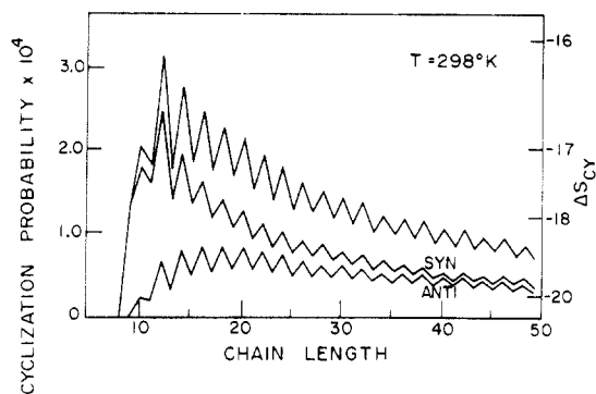
Figure 11. End-to-end cyclization probability W(O) for the molecules benzophenone- 4\text{CO}_2(\text{CH}_2)_m\text{NH}_2 , as a function of chain length. The data were obtained from a lattice-based RIS model employing Monte Carlo calculations. See ref 105e.
