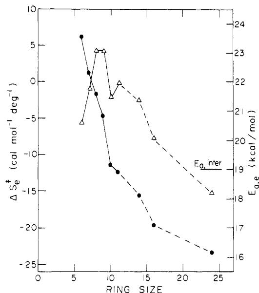
Figure 8. Activation energy E_{a,e} (right ordinate) and activation enthalpy \Delta S_{\ddagger,e}^{\ddagger} (left ordinate) for intramolecular catechol diether formation in o\text{-OC}_6\text{H}_4\text{O}(\text{CH}_2)_{n-4}\text{Br} as a function of ring size. The line E_{a,\text{inter}} refers to the activation energy of a corresponding bimolecular reaction. Data from ref 102.
