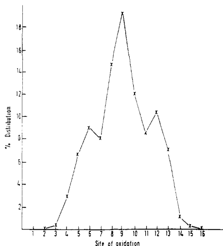
Figure 25. Percent oxidation of each of the \text{CH}_2 groups as a function of carbon number in the reaction of \text{CrO}_3 with hexadecanolate. From Eigendorf, Ma, and Money. 143
