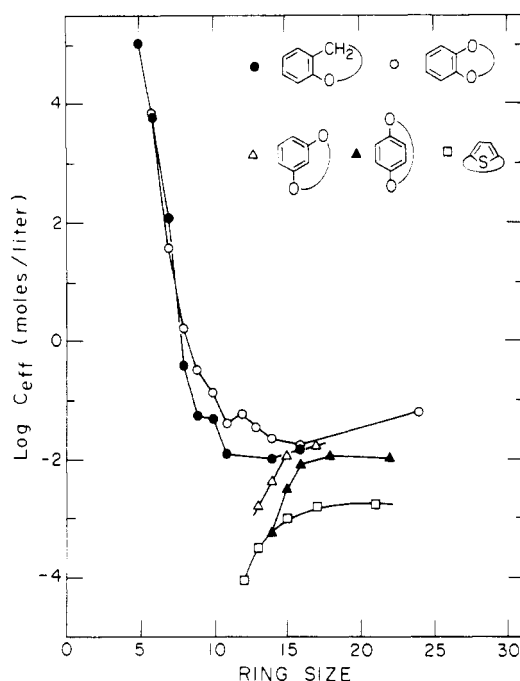
Figure 9. Effective concentration C_{\text{eff}} (moles/liter) plotted semilogarithmically vs. chain length for a variety of cyclization reactions whose kinetics were studied by Mandolini, Illuminati, and their co-workers. 104
