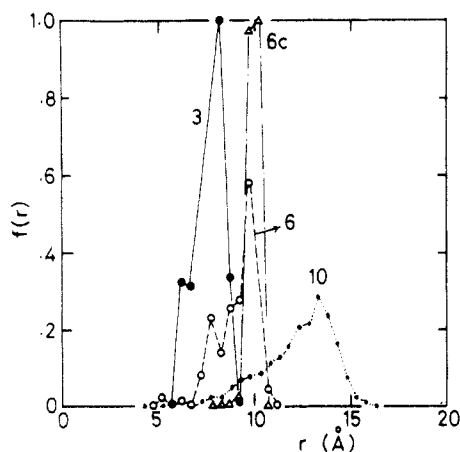
Figure 14. Distribution of the end-to-end distance r of N\cdot(\text{CH}_2)_n\cdot N from calculations based upon the RIS model. The numbers in the figure indicate the number of \text{CH}_2 groups n in the molecule. 6c = trans -1,4-bis(1-naphthylmethyl)cyclohexane. From ref 52.
